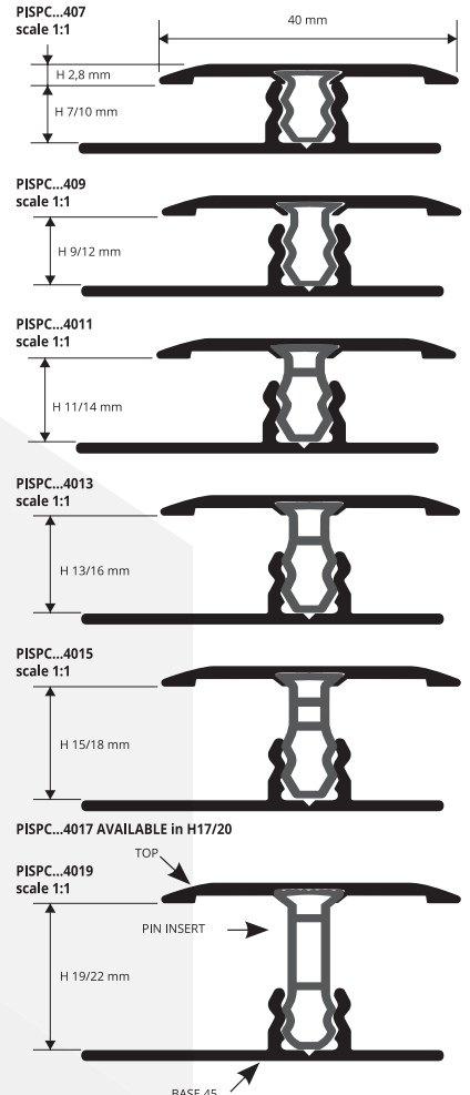
ALUM. TOP COVERED + PIN INSERT + ALUM. BASE 45 PUNCHED/PERFORED (80 wooden finishes of which 49 on demand) thermo packed bar length 2,7 lm - pack 20 Pcs - 54 lm (PIN 17, 19 - 40,5 lm)
